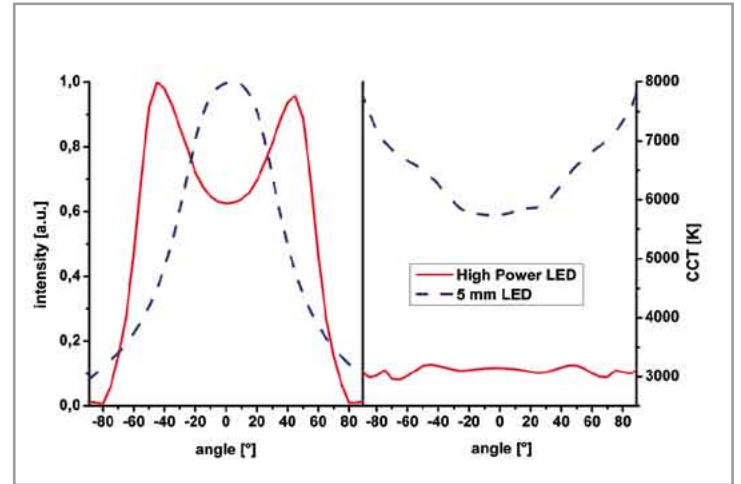
Figure 3: Spatial radiation pattern and color temperature of the emission of white light and standard LEDs, measured at a distance of 250mm
