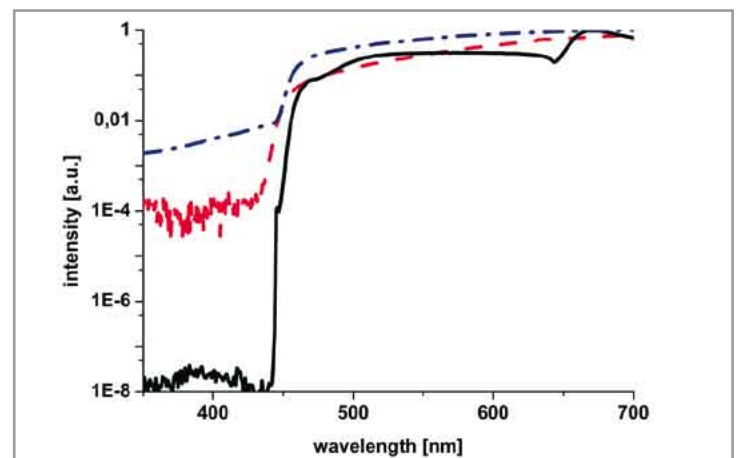
Figure 5: Stray light suppression for different spectrometers for filtered light from a halogen lamp: double monochromator (black), array spectrometer #2 (blue), array spectrometer #1 (red)
