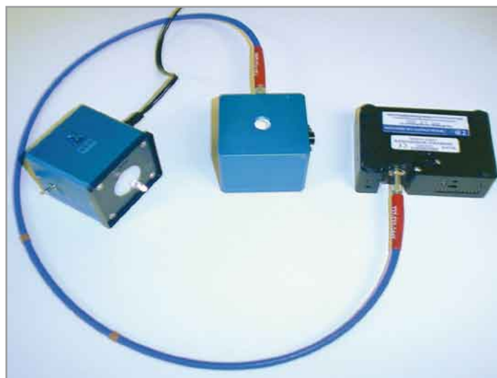
Figure 2: Typical LED characterization set-up with controlled NIST traceable power supply (left), integrating sphere (center) and fiber coupled miniature spectrometer (right)
