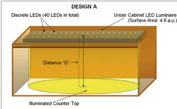
Figure 2: Design A Schematic showing a single luminaire of 4.8 a.u. surface area containing 40 LEDs
