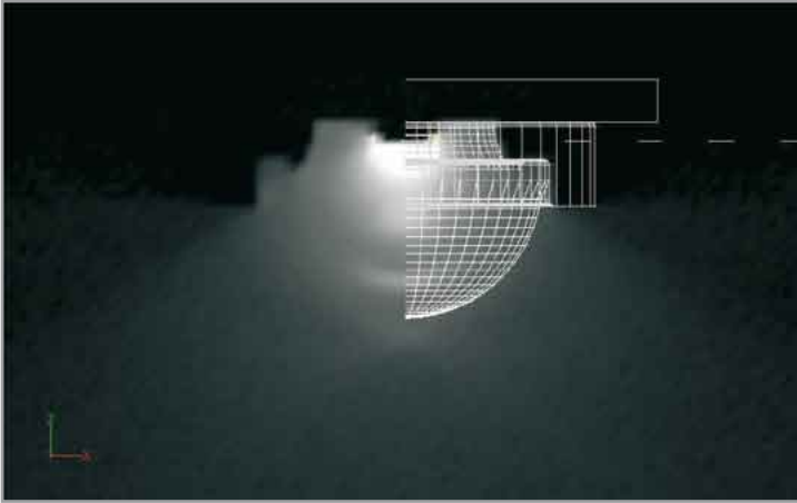
Figure 3: Type 3 Source Model
