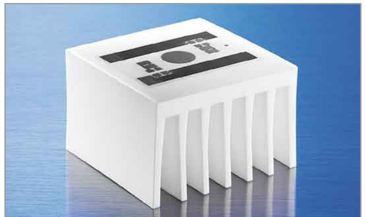
Optimized CeramCool® geometry for 4W cooling
