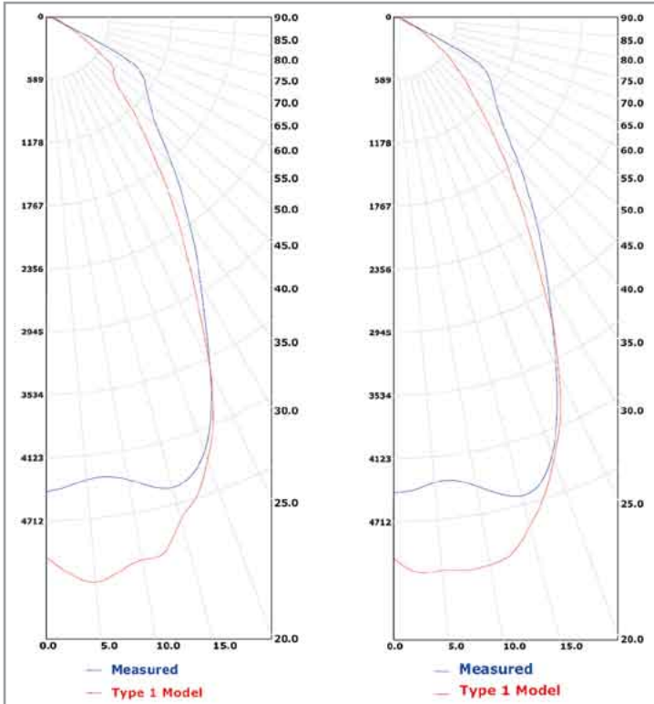
Figure 9: Type 1 Model Simulations: polar candela plots along chip (left) and diagonal to chip (right)
