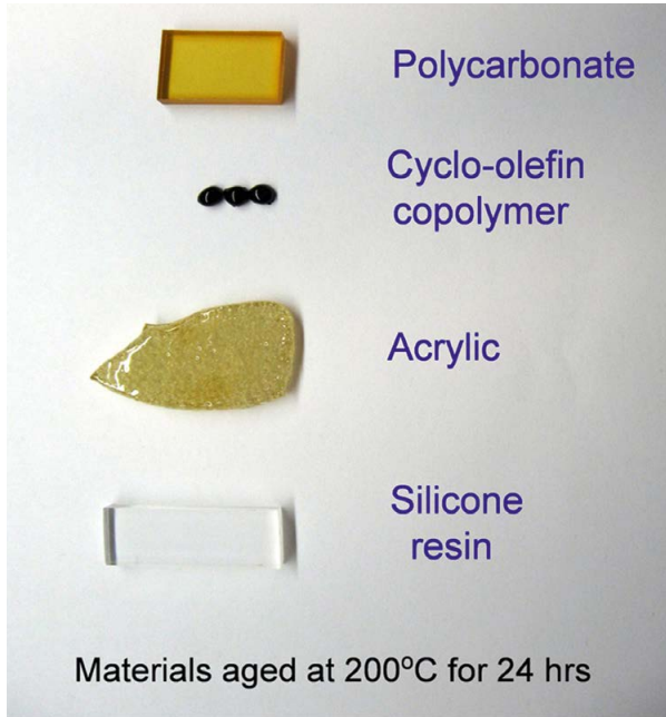
Figure 3: Comparative heat aging of polycarbonate, cyclo-olefin copolymer, acrylic and silicone resins after 24 hours at 200°C
