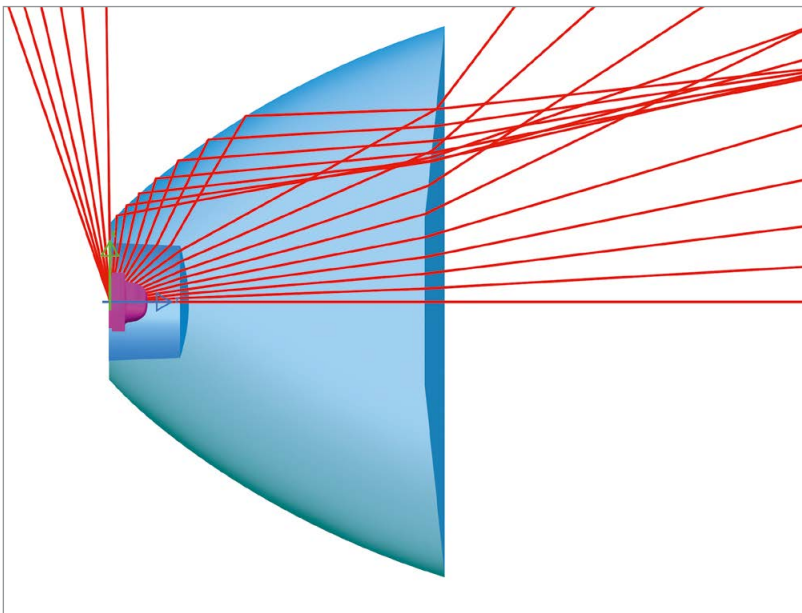
Figure 6: LED with emission >90^\circ with a TIR lens
