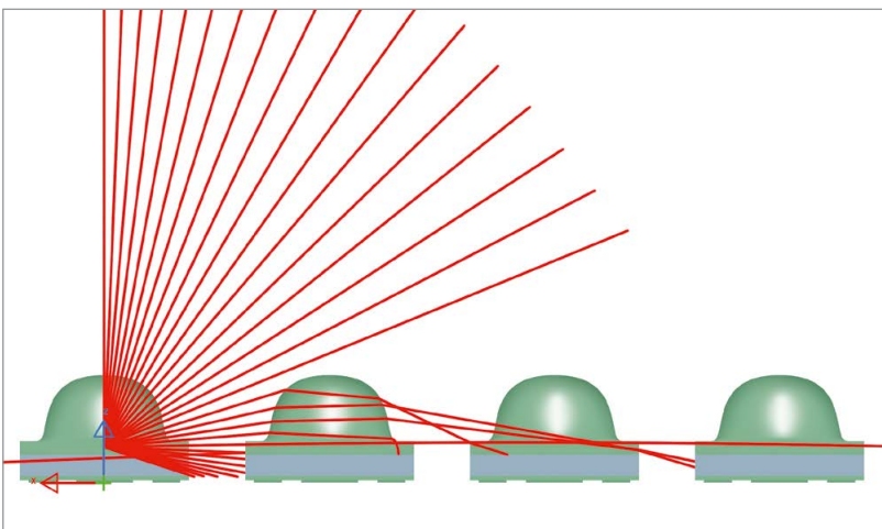
Figure 7: LED cluster with LEDs with an emission angle >90^\circ
