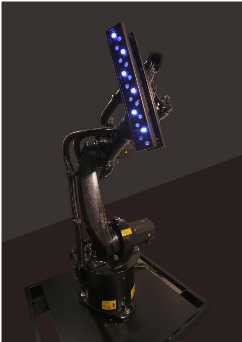
Figure 1: For LM-79 tests, luminous intensity distribution of luminaires is determined with goniophotometers
