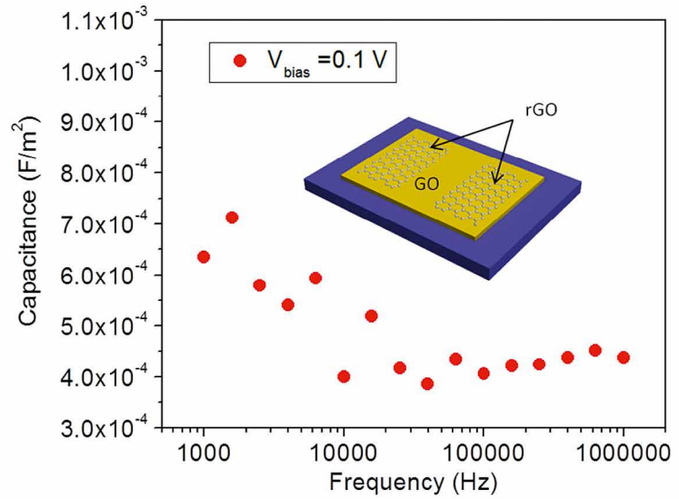
Supplementary Figure 5: Capacitance of GO dielectrics. C-f measurements were carried out on a Metal-Insulator-Metal structure. The two rGO regions were defined by laser-scribing as two capacitor electrodes, which in the GFLED act as the side gate and source electrode respectively
