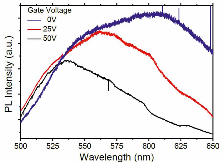
Supplementary Figure 7: Gate-Dependent PL of a typical GFLED
