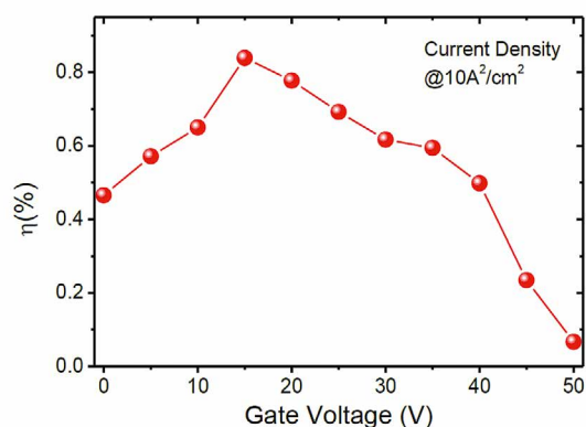
Supplementary Figure 10: Efficiency of a GFLED as a function of gate voltage
