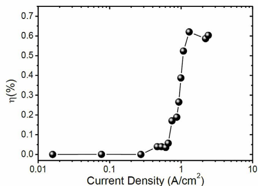
Supplementary Figure 9: Efficiency of a GFLED as a function of current density
