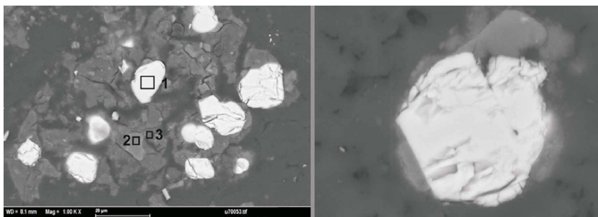
Figure 8: Material contrast image of coated phosphor material 1 particles 1000x BSE, 15 kV (left) and a single grain of coated phosphor material 1 at a magnification of 4000x BSE (right)
