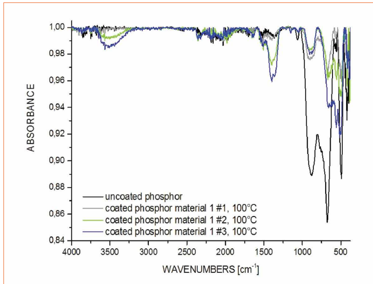
Figure 4: ATR-IR spectra of coated phosphor material 1 annealed at 100°C
