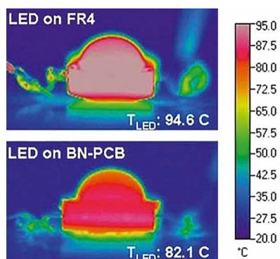
Figure 1: The images below show the thermal impact of LEDs and of other devices such as processors
