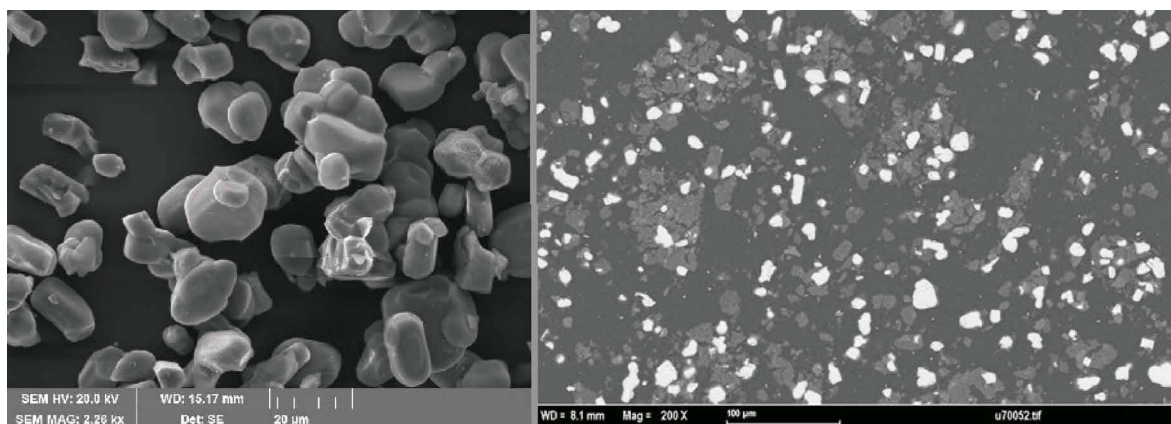
Figure 7: SEM image of uncoated phosphor material 1 at a magnification of 2.26kx (left) and a material contrast image of coated phosphor material 1, 200x BSE (right)
