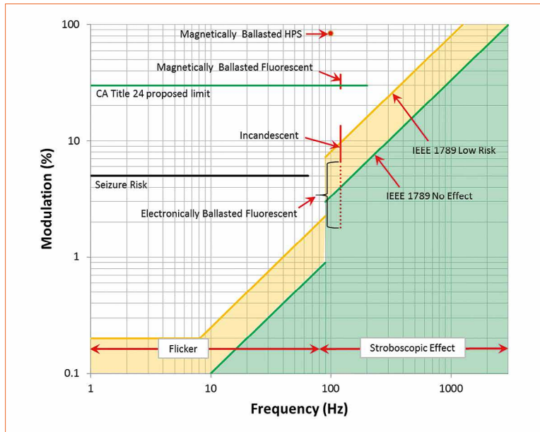
Figure 13: Flicker Modulation depth as a function of flicker frequency. Flicker modulation is given for no effect level (green) and low risk level (yellow)
