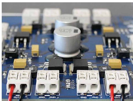
Electro Terminal has developed the Microcon SMD Power connector to provide direct mains voltage supply to electronic PCBs within a lighting system
