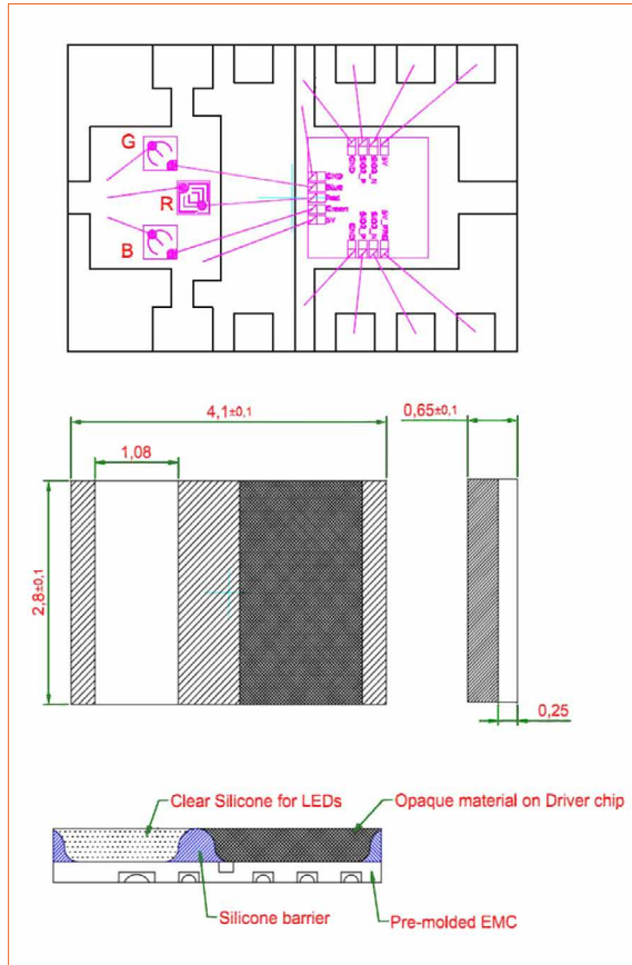
Figure 8: Compact packaging
