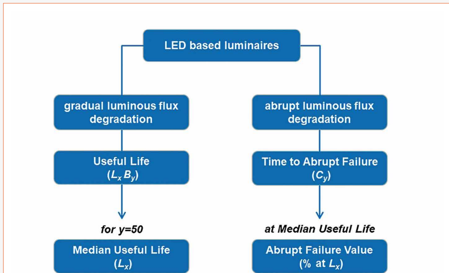
Figure 2: IEC lifetime metric
