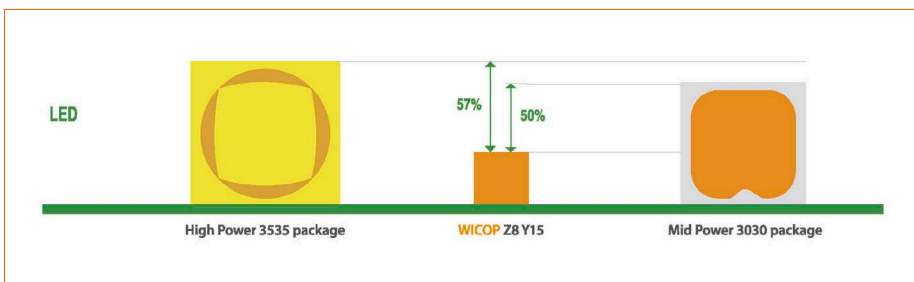
Figure 3: Size comparison of a traditional High-Power LED with WICOP and a Midpower 3030 LED
