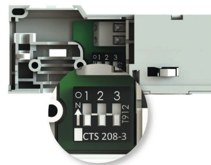
Figure 5: Simple setting of output current via dipswitch
