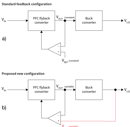
Figure 4: Standard feedback configuration a) and proposed new configuration b)
