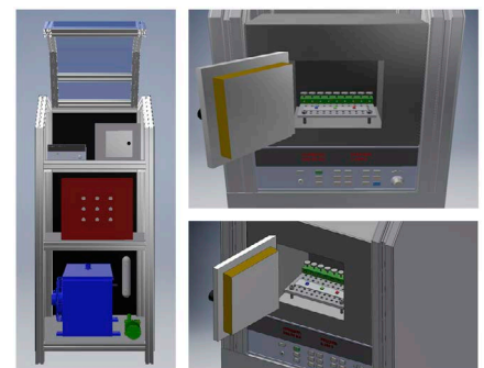
Figure 6: The assembly of all test units
