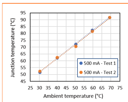
Figure 13: Evaluation of repeatability tests with a single blue LED driven at a 500mA operating current at different ambient temperatures
