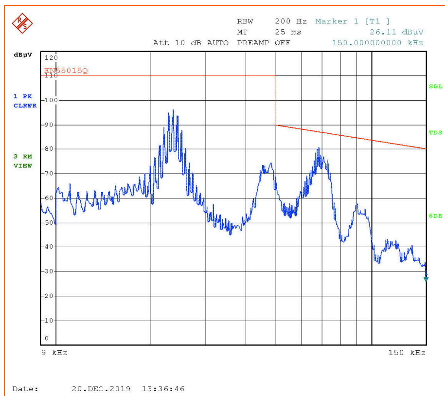
Figure 6: Extensive EMC measurements have been performed, both low and high frequency conducted and radiated
