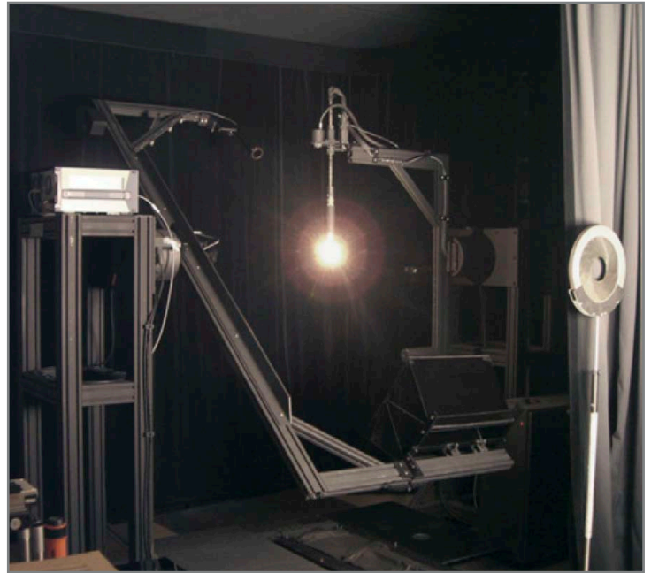
Figure 5: NIST gonio-spectroradiometer for the total spectral radiant flux scale realization
