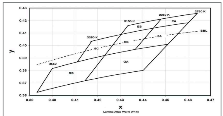
Figure 2: Warm White LED binning
