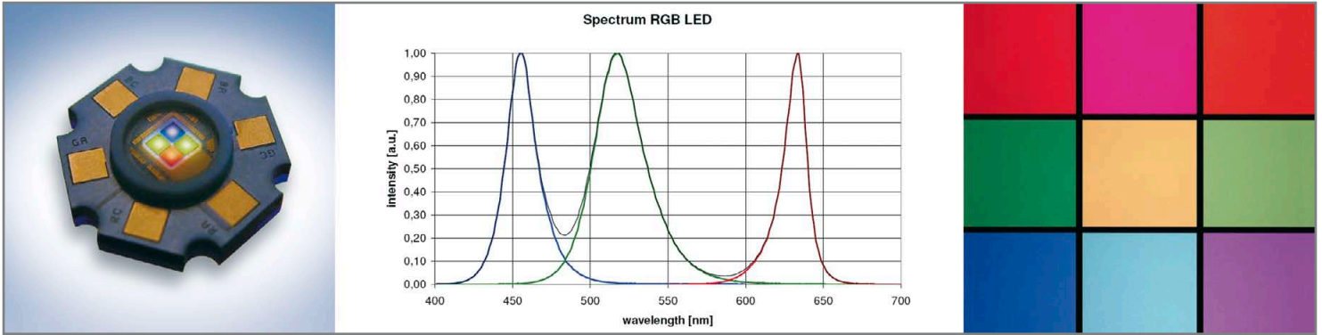
Figure 9: RGGB LED ACULED (left): Spectrum (middle) and color rendering (right)
