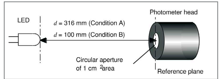
Figure 1: Geometry for CIE Averaged LED Intensity
