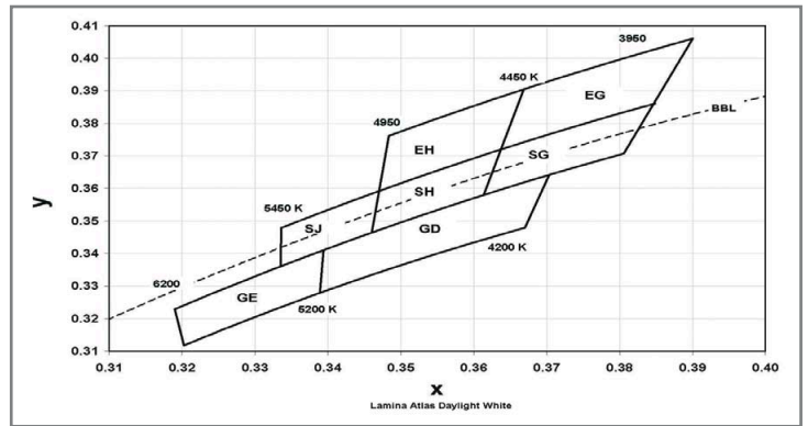
Figure 1: Cold White LED binning
