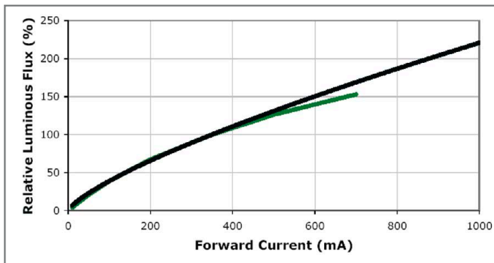
Figure 3: Relative Flux vs. Current @ Tj = 25°C from the data sheet
