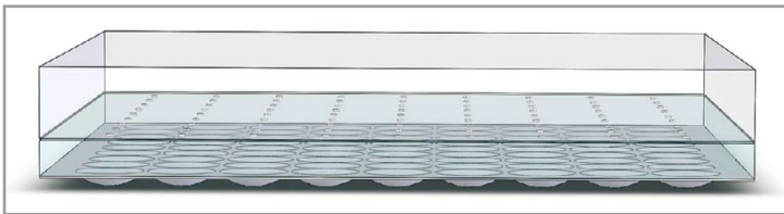
Figure 3: A hierarchal waveguide basically consisting of the LED coupling, the primary waveguide with attached secondary waveguide using a transparent coupling medium with embedded secondary emitters, a diffusion layer and a micro-collimator array
