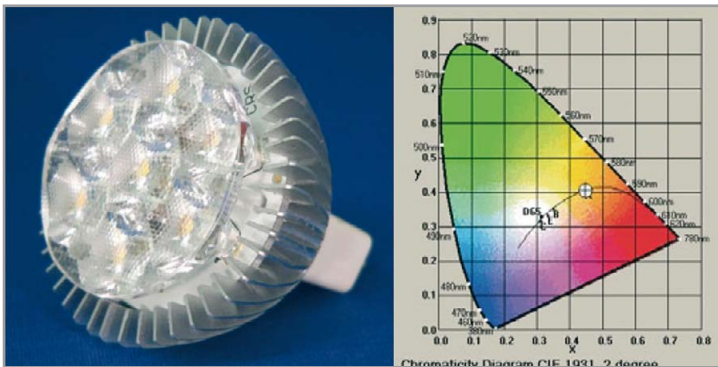
The CRS MR16 replacement lamp that achieved a 325lm@2800K
