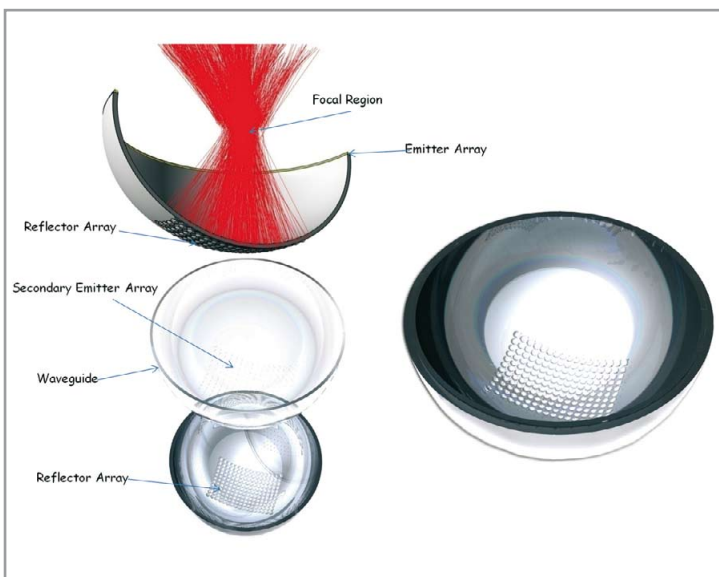
Figure 5: An example of concave illuminator design
