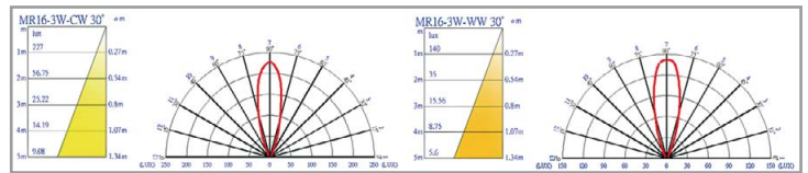
MR16 LED candlepower distribution curve (1m)
