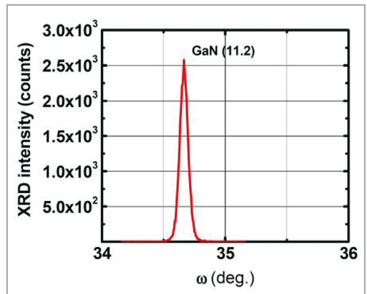
XRD w-scan rocking curve
