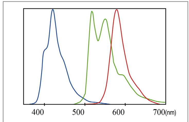
Figure 5: Typical white light OLED spectrum.
