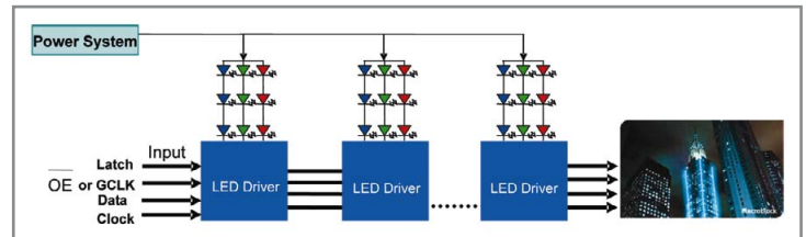
Figure 2: The traditional four-wire transmission.
