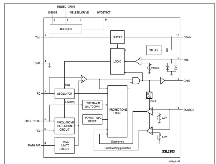
Block diagram of the SSL2103 mains LED driver with external switches for high power applications.
