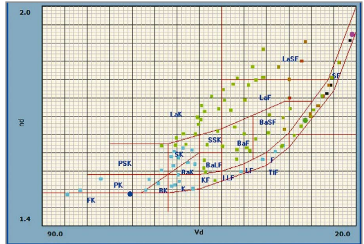
Figure 1: n/V-value plot, so-called Abbe-diagram.
