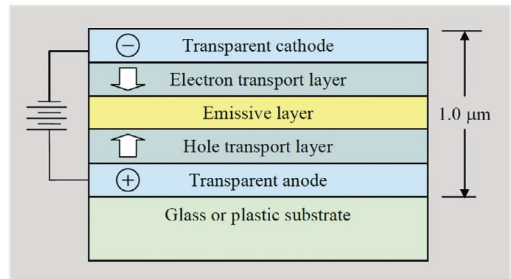
Figure 1: Typical OLED device
