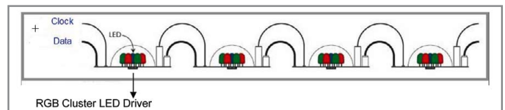
Figure 3: Two-wire transmission with Clock and Data signals.
