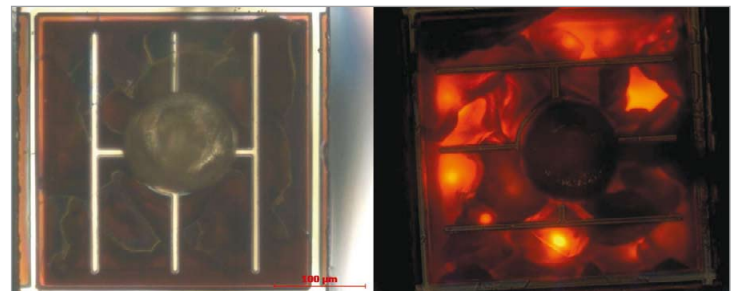
Figure 2: Reflected light (left) and transmitted light (right) microscopy of a typical surface corrosion.
