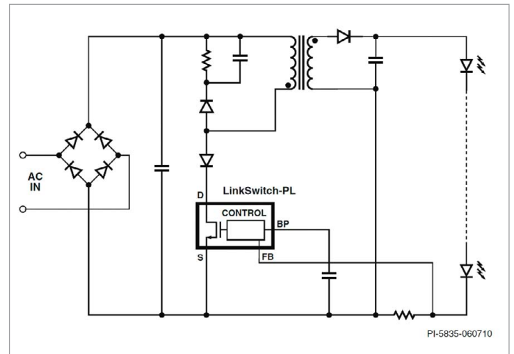
Basic application schematic with LinkSwitch-PL.
