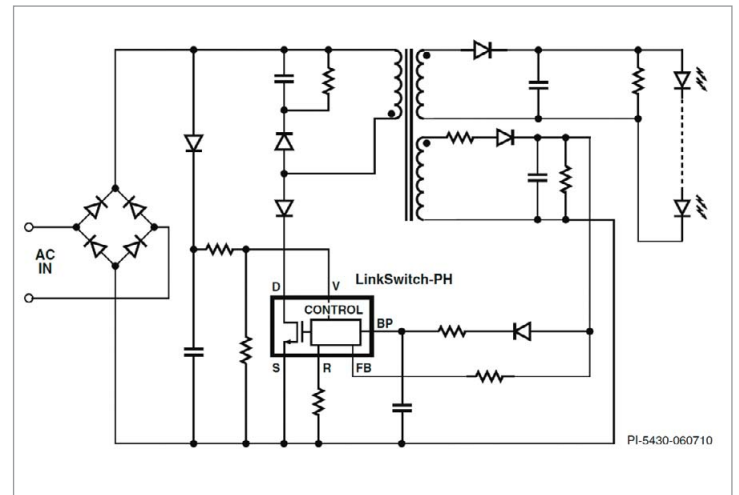
Typical application schematic with LinkSwitch-PH.
