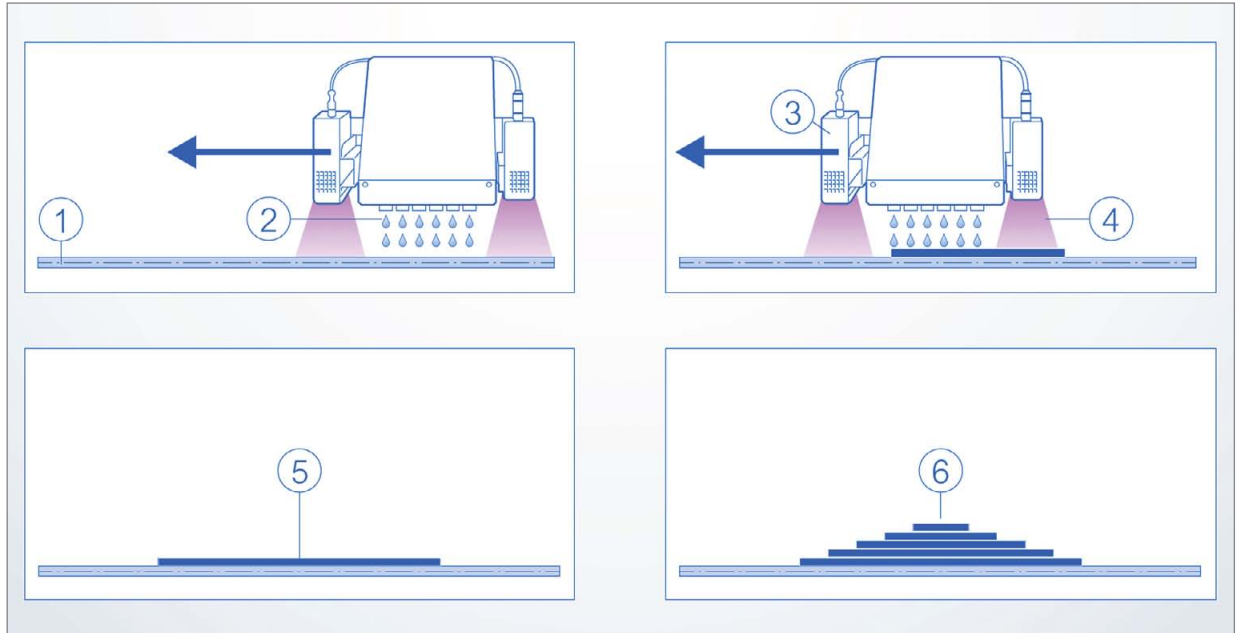
Figure 2: Schematic representation of the four stages in print-optical technology: 1. Substrate 2. Spraying dots of UV-curable polymer 3. UV-LED source 4. UV beam 5. First layer of polymerized bubbles 6. Stacked layers of bubbles
