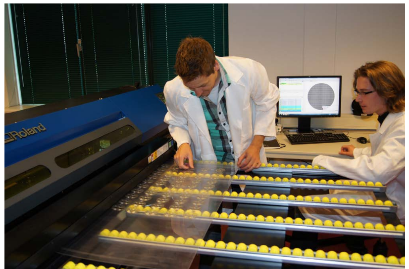
Figure 1: Making optical products with print-optical technology on a modified Roland printer. The yellow rollers are for guiding the substrate
