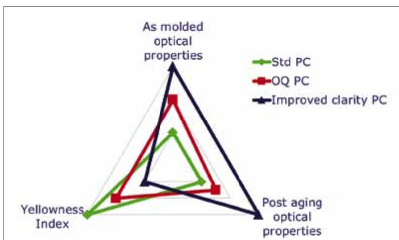
Figure 1: Improvements in polycarbonate from standard PC to Optical Quality PC to Improved Clarity PC when positioned for LED applications. Superior optical properties (as molded and post aging – thermal and UV) with lower Yellowness Index is desirable
