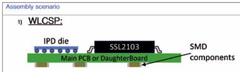
Example of a realization based on LED Driver
