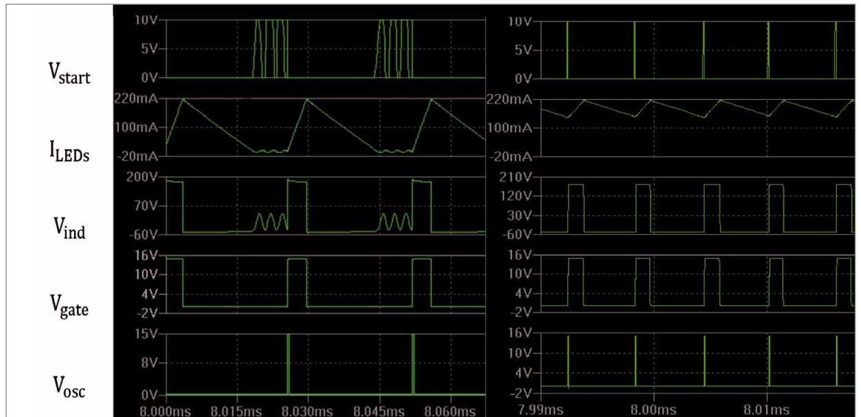
Figure 3: Simulated waveforms of the drivers shown in Figure 1 and 2. On the left, the basic driver is sourcing low output current in DCM. On the right the modified driver circuit is sourcing the same output peak current and operating in BCM
