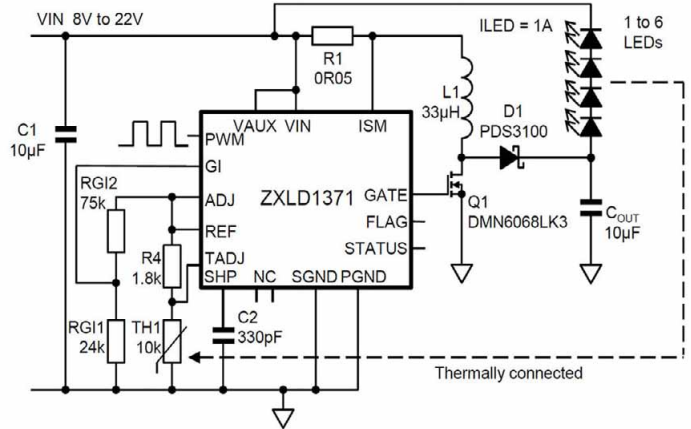
Typical application diagram for buck-boost solution utilizing a thermistor and TADJ
