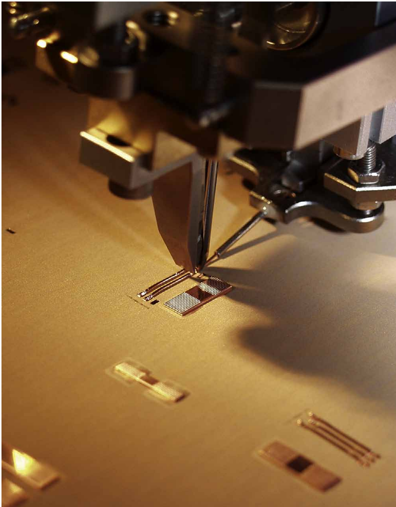
Figure 2: Exterior copper components within the type of wires or profiles are deposited directly onto the base copper by means of ultrasonic welding
