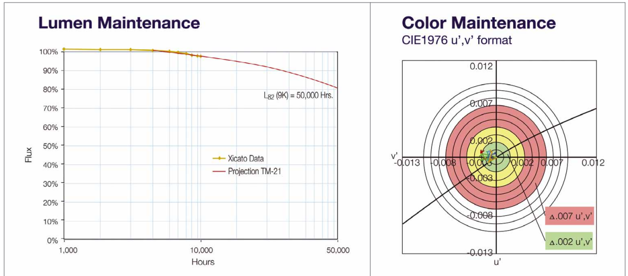
Figure 5: Lumen and color maintenance data
