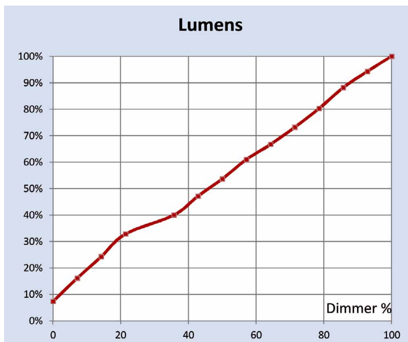
Figure 4: Typical dimming curve of AC LEDs on both leading edge or trailing edge phase cut dimmers: Phase cut dimming removes part of the AC waveform by switching on and/or off during each repetition of the 50 or 60 Hz current cycle. If the cycle is held off until switched on, this is leading edge phase cut. If the cycle is switched off part way through, this is trailing edge phase cut
