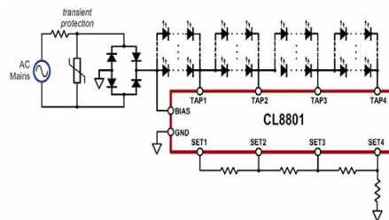
Typical application circuit using the CL8801 which has four current regulator outputs
