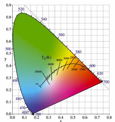
Figure 2: CIE 1931 diagram
