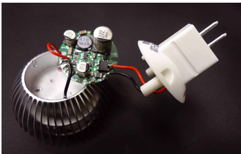
Figure 1: Typical electronics that is used to drive DC LEDs, in this case from an MR16 lamp
