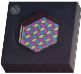
MAZeT's new color sensor MTCSiCF for photometry is placed in a newly designed housing
